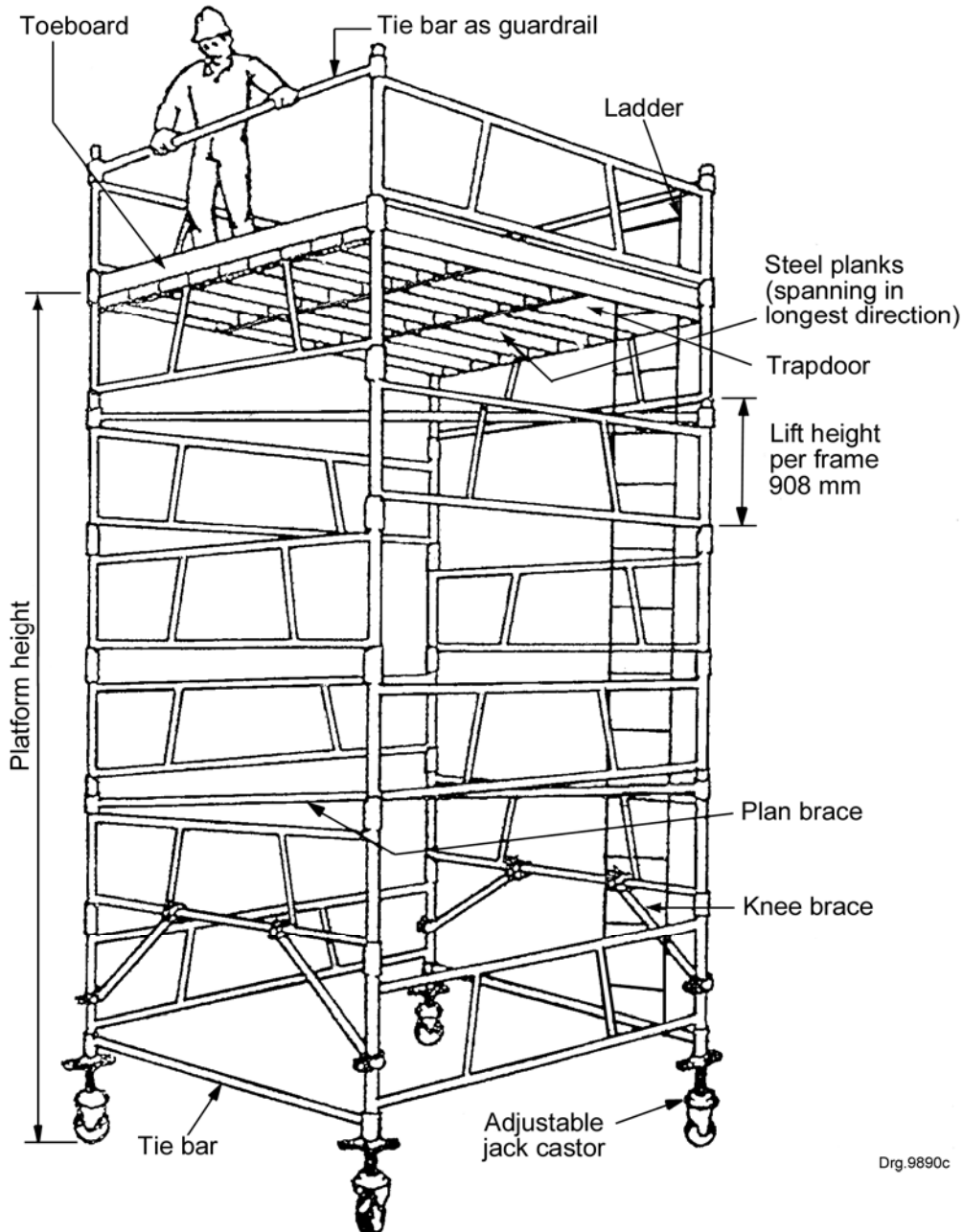
Figure 1 — Tubular steel mobile tower (interlocking frame scaffolding)
